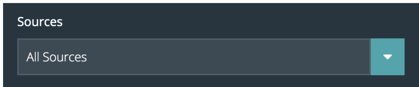
Figure 7. Select Sources
